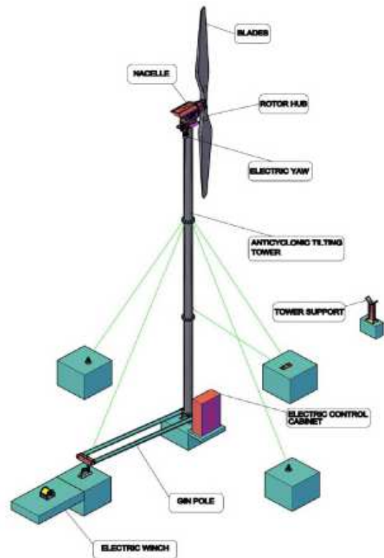
Tilt-tower (optional)
